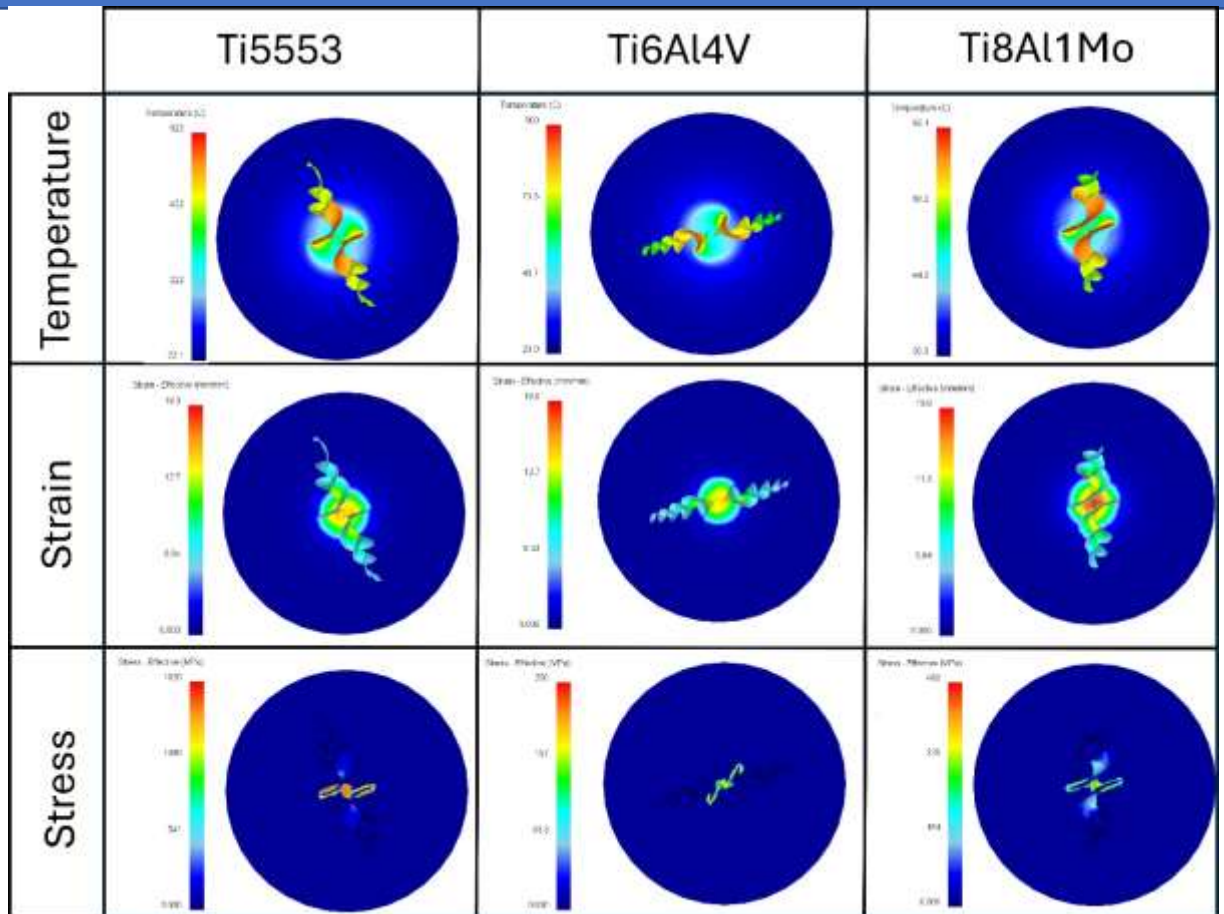
Figure 3. Temperature, strain and stress distributions obtained for titanium alloys
