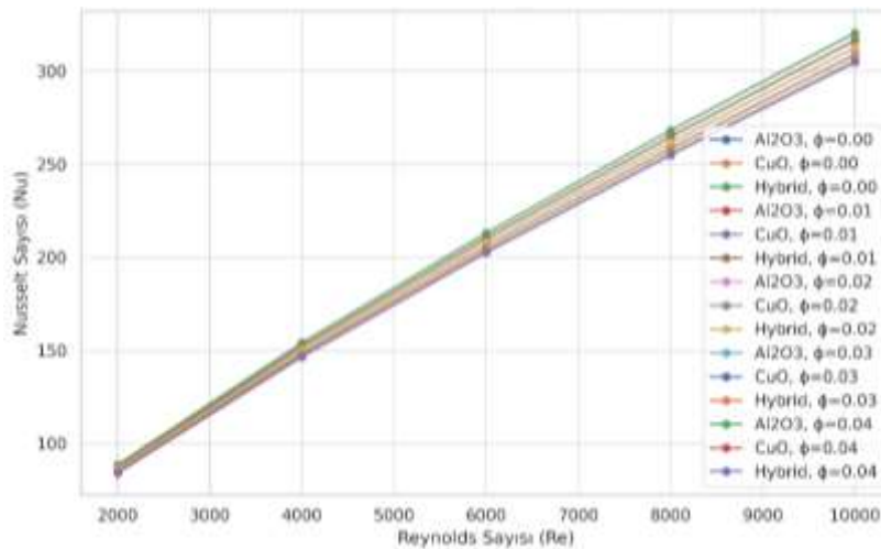
Figure 1. Variation of Nusselt number with Reynolds number for Al_2O_3 , CuO , and hybrid nanofluids at different particle volume fractions ( \phi = 0.00–0.04 ).
