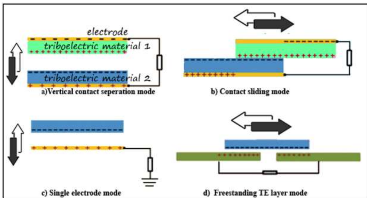
Figure 2. Basic working modes of TENG systems
