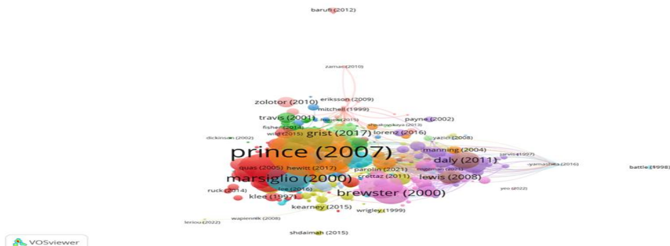
Figure 6. Bibliographic coupling of documents
