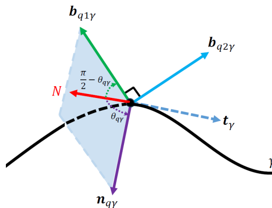
Figure 4. Case N \in Sp\{n_{q\gamma}, b_{q1\gamma}\} for curve \gamma
