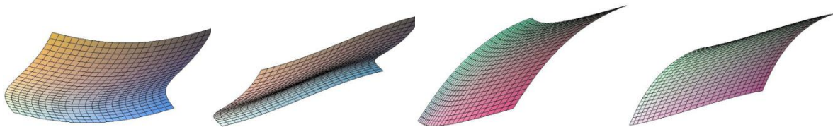
Figure 6. Translation surfaces in xyz , xyt , xzt and yzt -spaces
