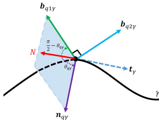
Figure 3. Case N \in \text{Sp}\{\mathbf{n}_{q\gamma}, \mathbf{b}_{q1\gamma}\} for curve \gamma
