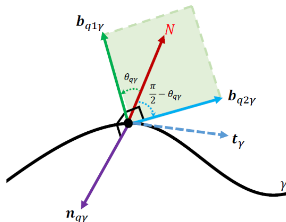
Figure 5. Case N \in Sp\{\mathbf{b}_{q1\gamma}, \mathbf{b}_{q2\gamma}\} for curve \gamma
