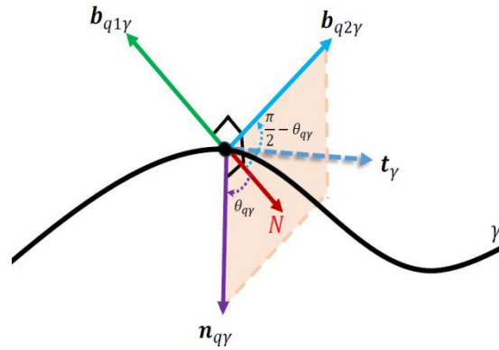
Figure 4. Case N \in Sp\{\mathbf{n}_{q\gamma}, \mathbf{b}_{q2\gamma}\} for curve \gamma
