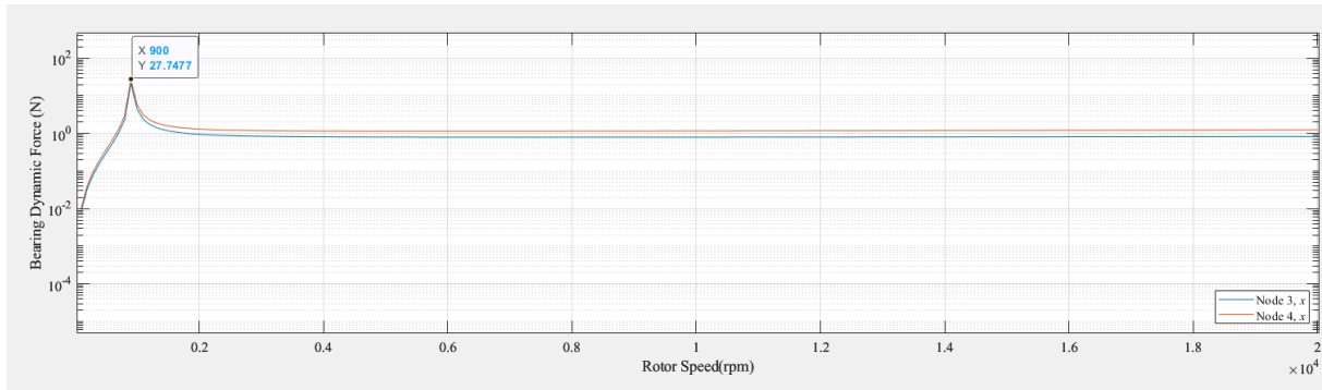
Figure 6. Bearing Dynamic Force vs Rotor Speed(rpm)
