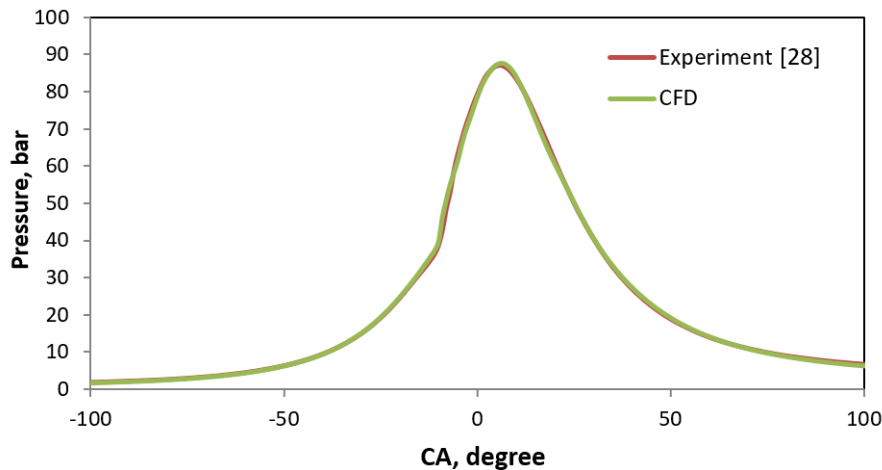
Figure 2. Validation of CFD model with experimental pressure data
