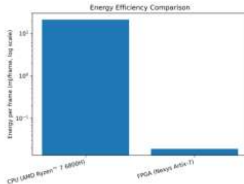
Figure 7. Energy consumption per frame comparison between CPU- and FPGA-based solutions
