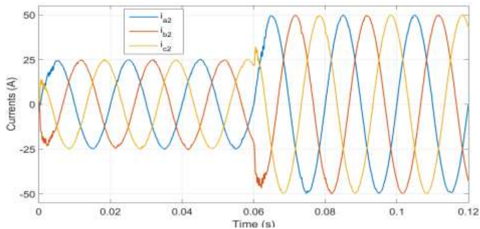
Figure 4. Currents transferred to the grid ( i_{abc2} ).
