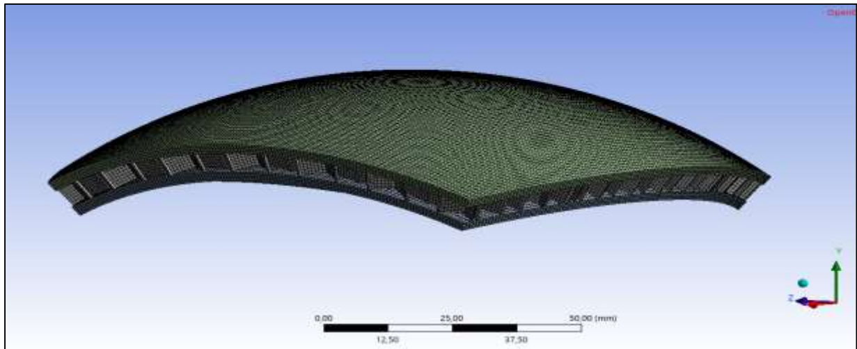
Fig. 3. Visualization of the sandwich shell in the first mode.
