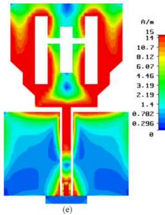
Fig. 6: Current distribution of the proposed antenna at (a) 2.4 GHz (b) 2.5 GHz (c) 3.5 GHz (d) 5.25 GHz and (e) 5.5 GHz.
