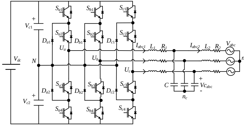
Figure 1. Three-phase, three-level, three-leg, three-wire, grid-connected, LCL filtered NPC inverter circuit.
