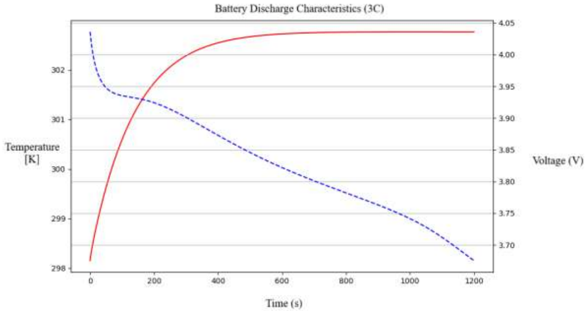
Fig. 4. Battery Discharge Characteristics (3C), Time-dependent variation of Temperature and Voltage.
