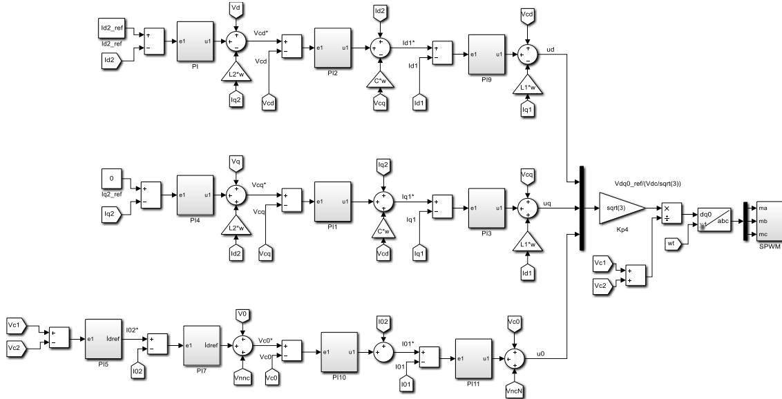
Figure 3. MATLAB model of the control system proposed for the control of the inverter circuit.
