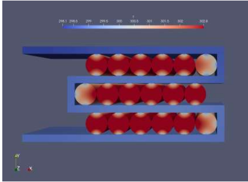
Fig. 3. Temperature distribution obtained in the batteries at the end of the 3C discharge (1200 seconds) resulting from cooling with the BN-water mixture coolant.
