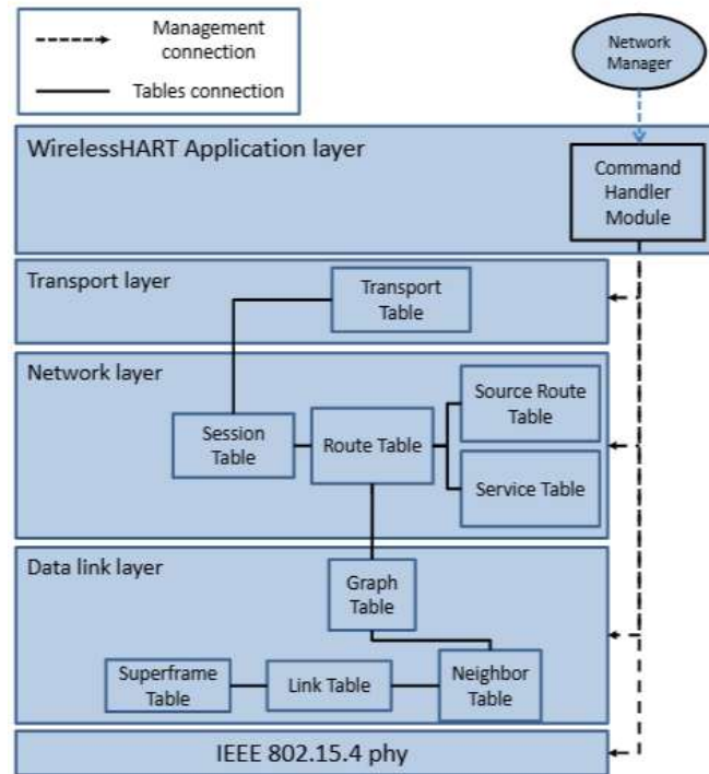
Fig.3. The layer of WirelessHART
