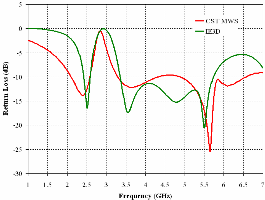
Fig. 4: Comparative study of proposed antenna in CST and IE3D EM Simulator.
