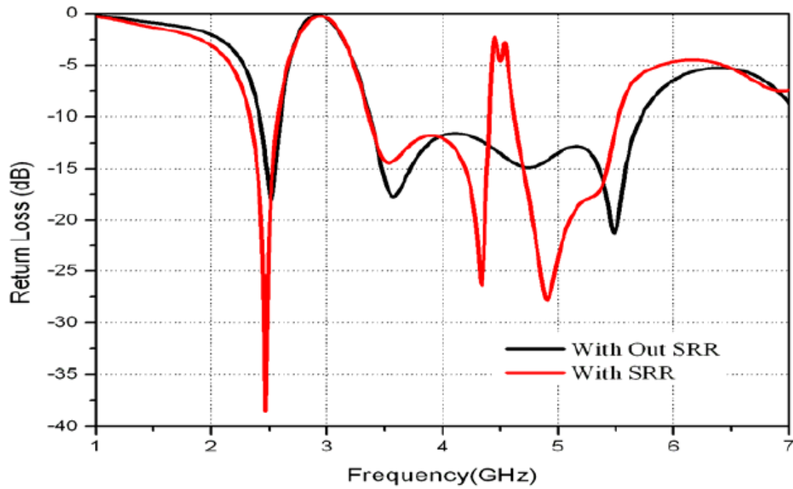
Fig.10: Return Loss characteristics of proposed SRR embedded antenna compared with simple planar monopole antenna.
