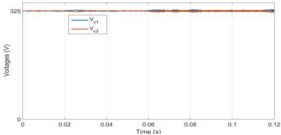
Figure 8. The voltages of DC bus capacitors ( V_{c1} , V_{c2} ).
