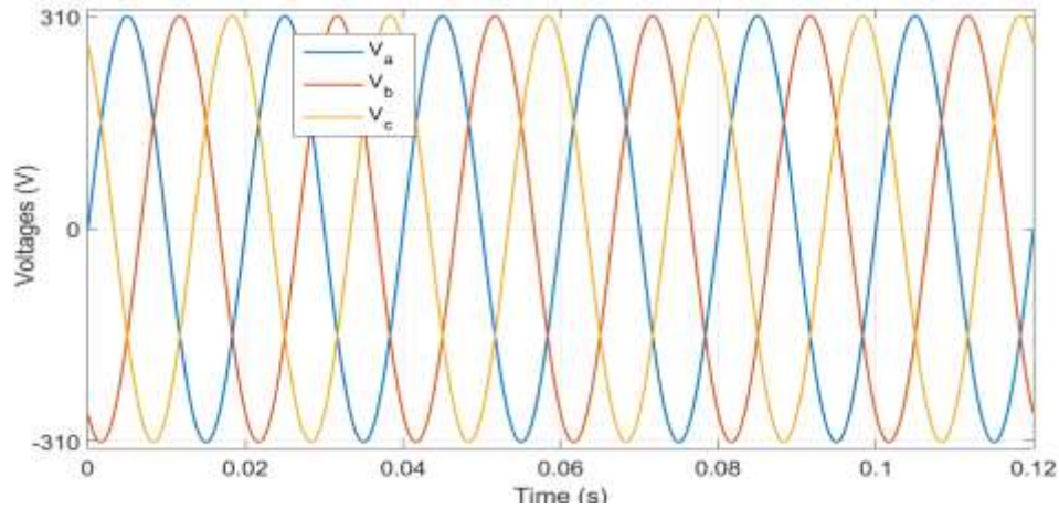
Figure 5. Grid voltages ( V_{abc} ).
