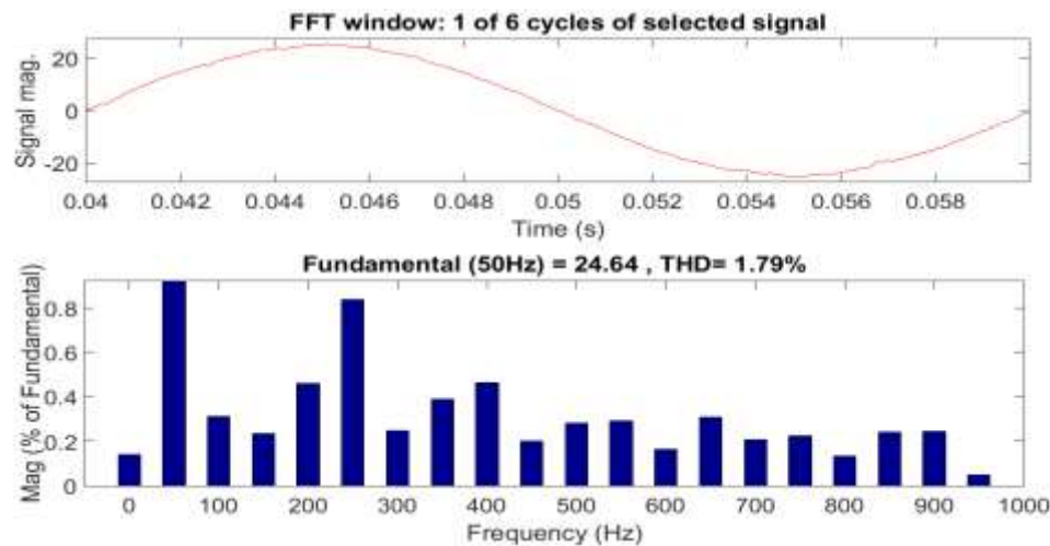
Figure 6. FFT analysis of the grid current while the magnitude of the current is 25 A.
