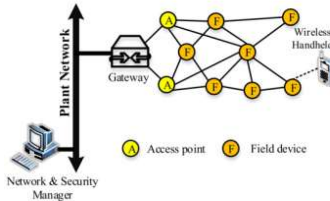
Fig.2. The mesh topology in WirelessHART
