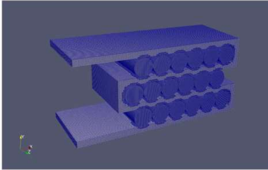
Fig. 1. Three-dimensional computational mesh of the battery module generated using the snappyHexMesh utility, depicting the discretization of the solid and fluid regions.
