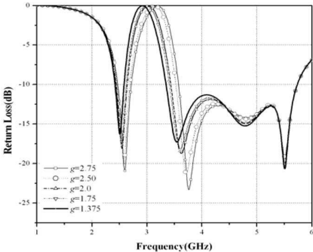
Fig. 3: Return Loss Characteristics of proposed antenna for parametric study by varying g . Other parameters are w_1=w_2=w_3=3.1 , (l'_1+l_2)=(l_1+l_2)=18.4 , (l_3+l_4)=12.5 . (All dimensions in mm)
