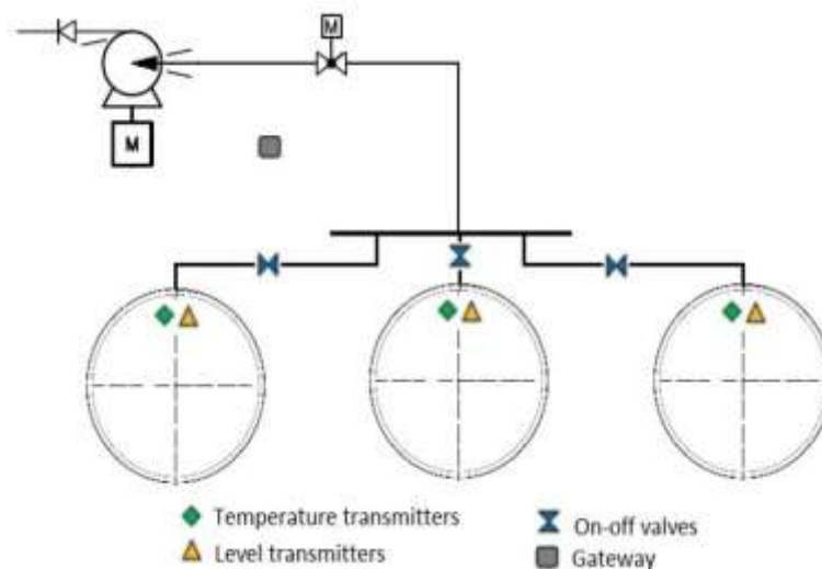
Fig.7. The system diagram
