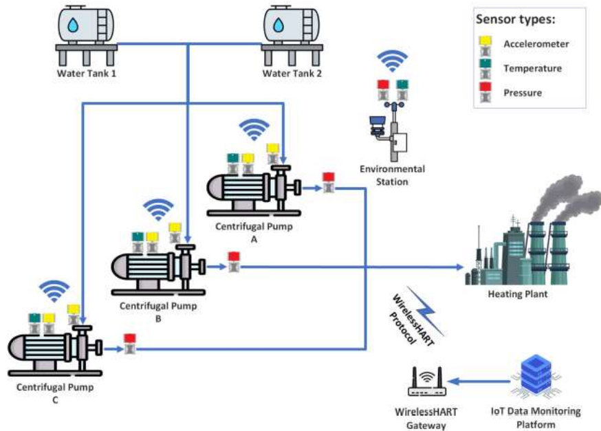
Fig.9. Schematic representation of the target plant and the WirelessHART architecture.
