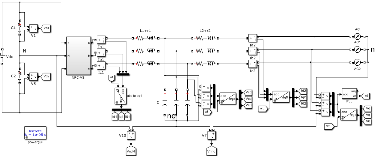
Figure 2. MATLAB model of a three-phase, three-level, grid-connected NPC inverter with LCL filter.
