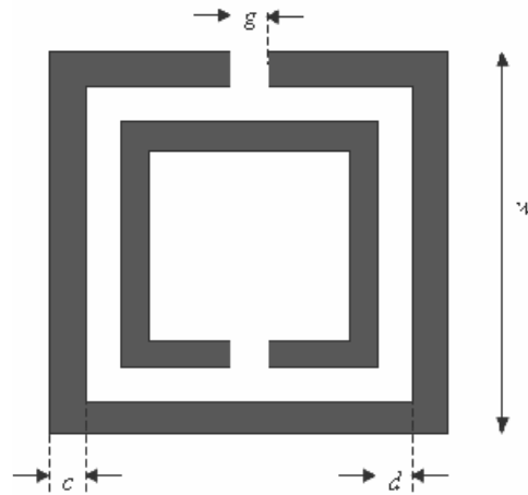
Fig. 7: Geometry of proposed SRR unit cell.
