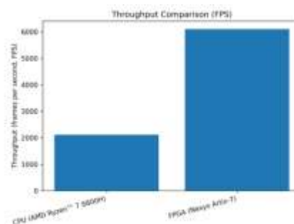
Figure 6. Frame rate (FPS) comparison between CPU- and FPGA-based solutions
