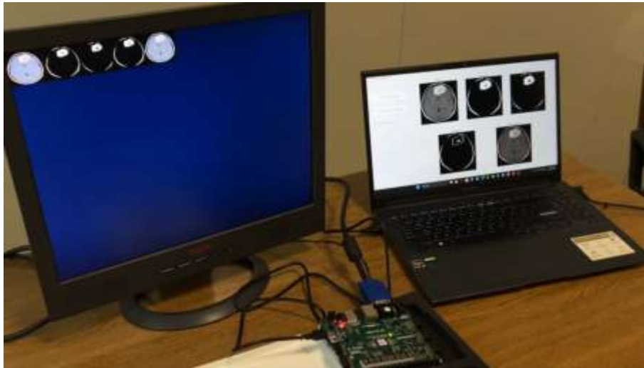
Figure 9. Real-time image processing results obtained via the VGA output on the FPGA
