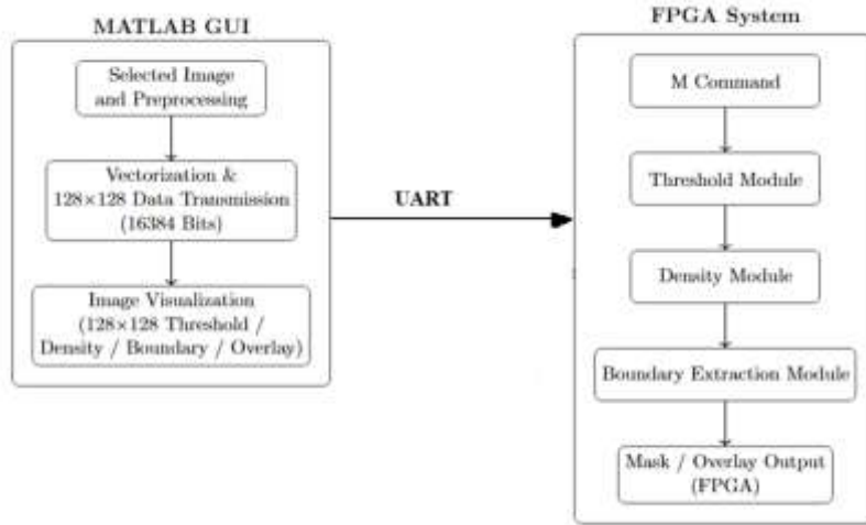
Figure 2. MATLAB–FPGA communication structure
