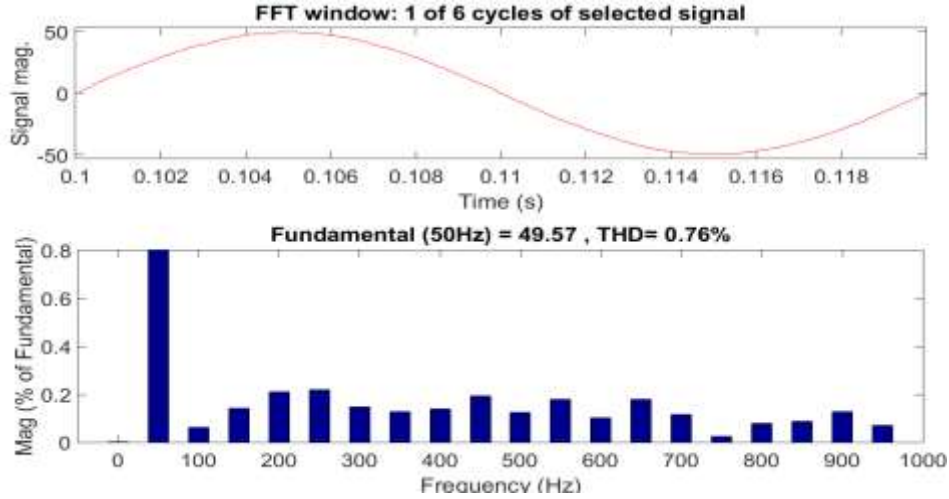
Figure 7. FFT analysis of the grid current while the magnitude of the current is 50 A.
