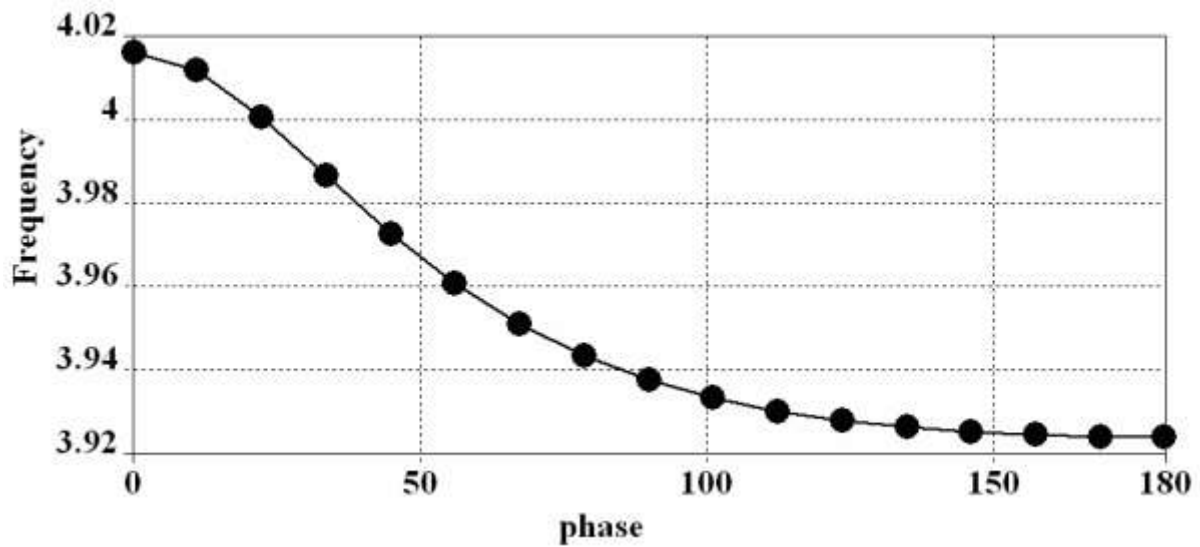
Fig. 8: The negative dispersion characteristics of proposed SRR
