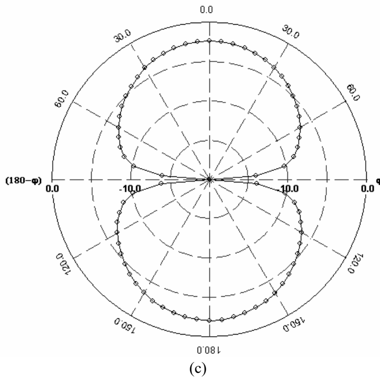
Fig.11: The elevation plane radiation pattern of proposed antenna (a) 2.4 GHz (b) 3.5 GHz (c) 5.25GHz
