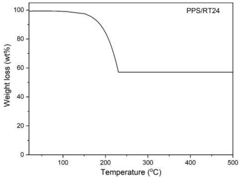
Figure 4. TGA curve of PPS/RT24
