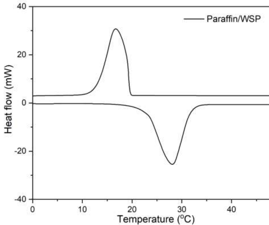
Figure 3. DSC curve of Paraffin/WSP composite
