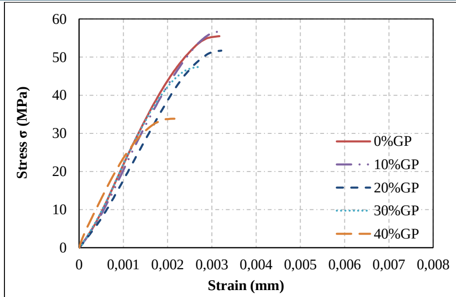
Figure 4: Effect of GP on stress - strain relation for 0.4 w/b concretes
