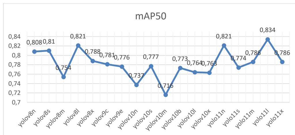
Fig. 2. mAP50 results of the models.
