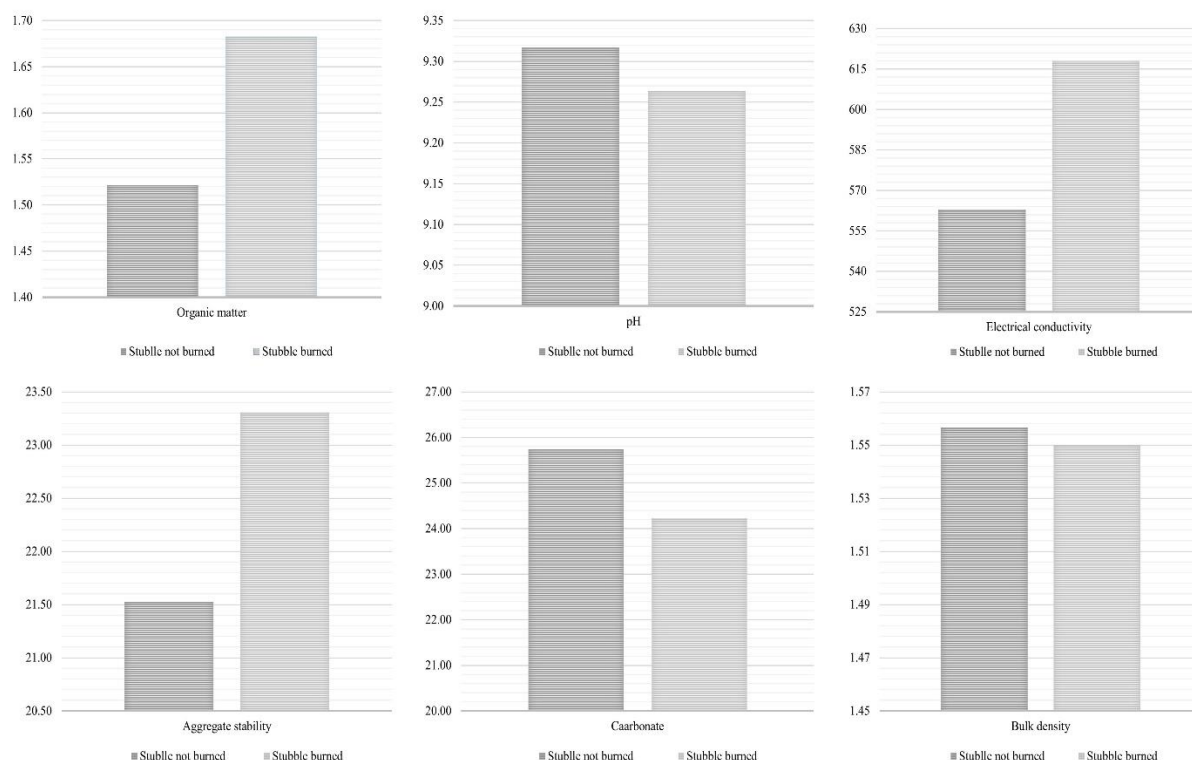
Figure 3. Organic matter (%), pH, aggregate stability (%), lime (%), electrical conductivity ( \mu\text{mhos} \cdot \text{cm}^{-1} ) and bulk weight ( \text{g} \cdot \text{cm}^{-3} ) values of soils according to sampling time and applications.
