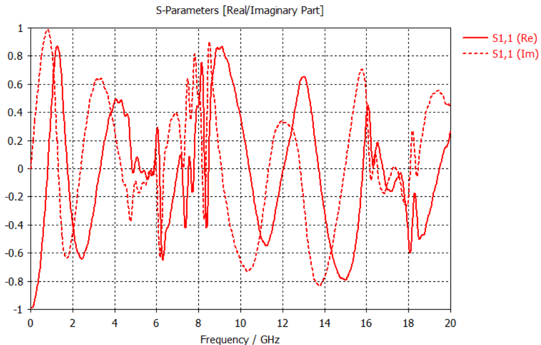
Figure 3. Real and imaginary parts of S_{11}(\text{dB})
