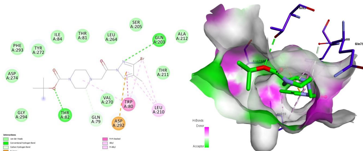
Figure 1. 2D and 3D interactions of the pyrazole 2 and 4EJN complex
